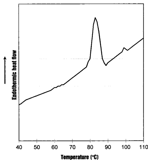
Figure 3. DSC thermogram of rice bran protein isolate (RBPI).
